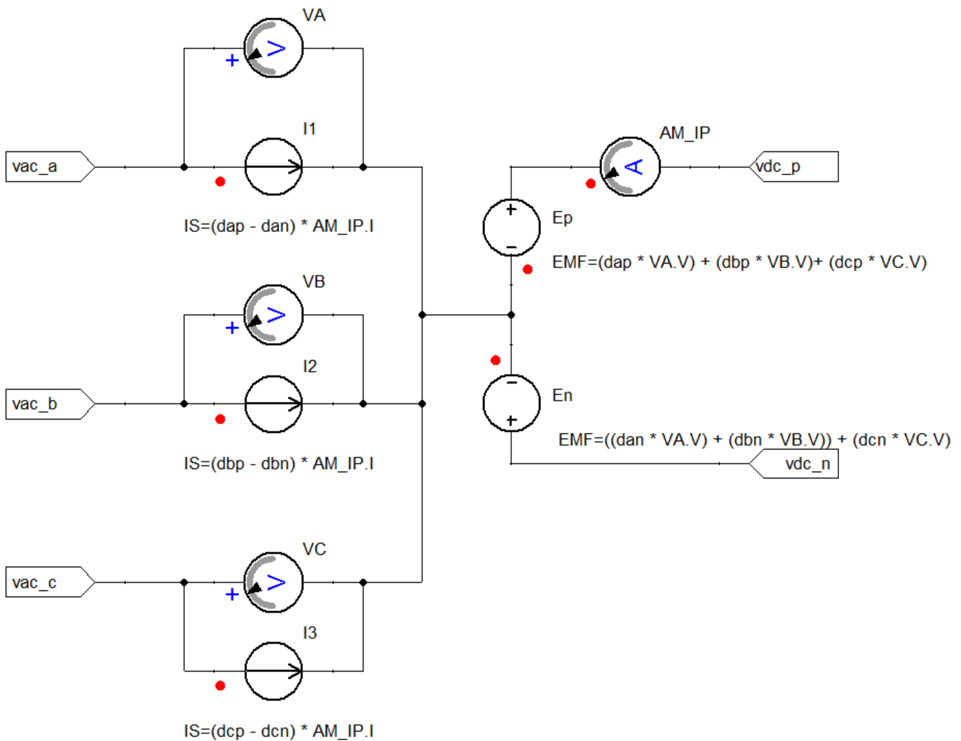
Figure 2. Equivalent Circuit Schematic
