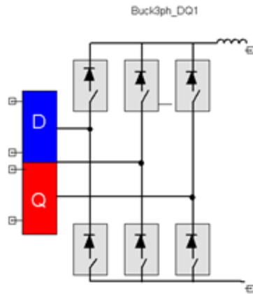
Figure 1. Component symbol
