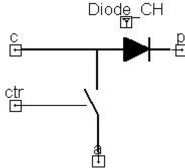
Figure 1. Component symbol
