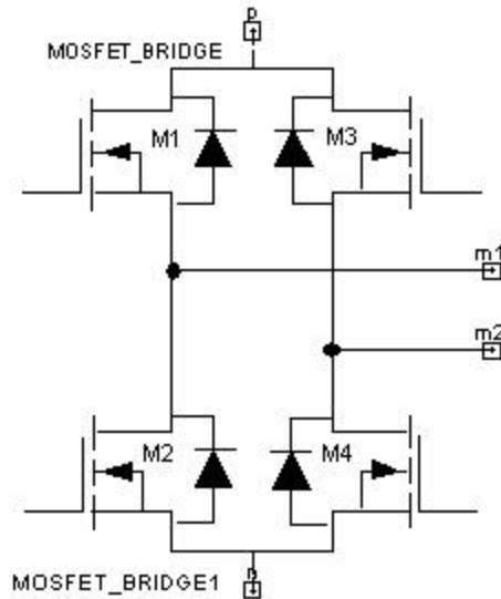
Figure 1. Component symbol
