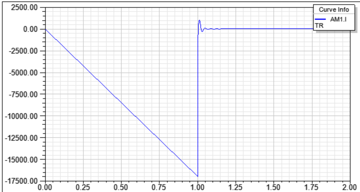
Figure 3. Simulation results – Source Output Current (AM1.I) showing circuit breaker tripping at 1ms.
