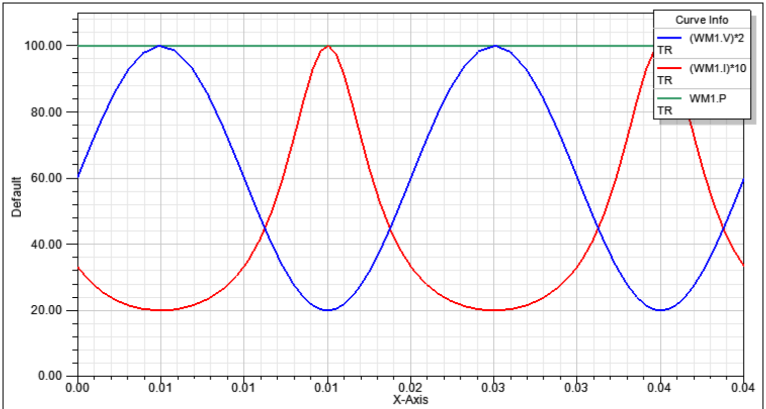
Figure 3. Simulation results-Voltage (WM1.V*2), Current (WM1.I*10) and Power (WM1.P) measured by the power meter.
