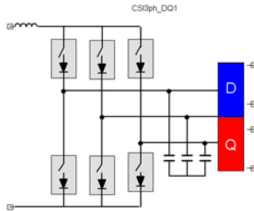
Figure 1. Component symbol
