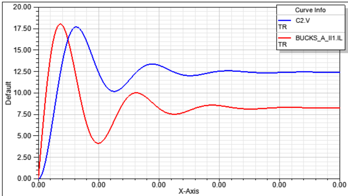
Figure 4. Simulation results-Output current (BUCKS_A_II1.IL), and Output Voltage (C2.V).
