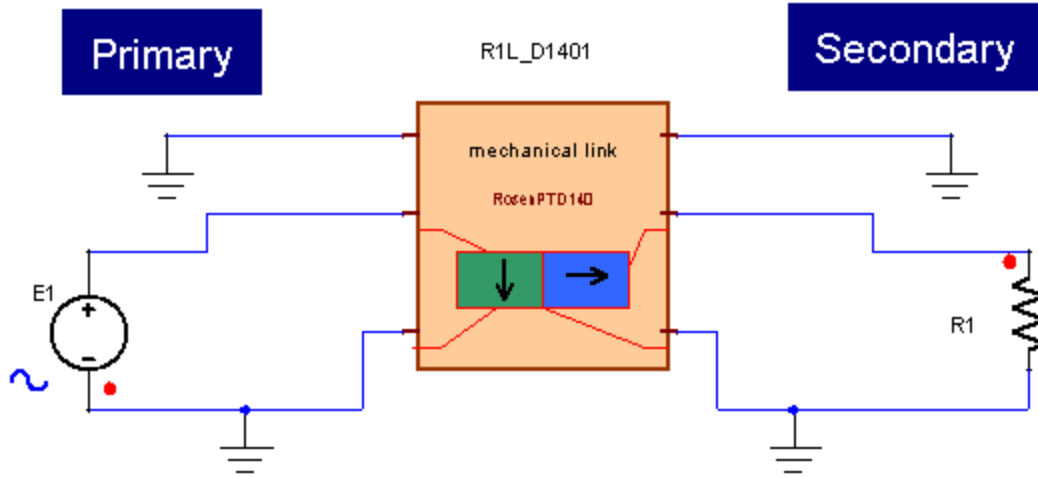
Figure 2. Application example of the Rosen Monolayer R1L_D140 model
